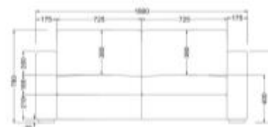
2.5 SEATER DX-LZR-2.5-DS 1800(L) X 860(W) X 400(SH) X 780(H)
